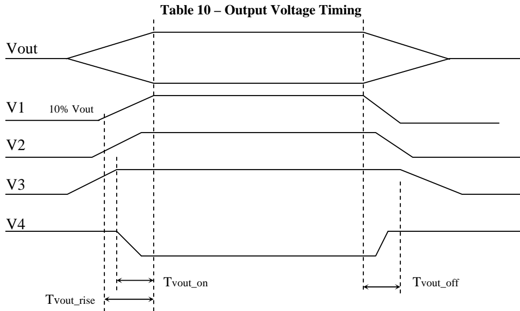
Figure 1: Output Voltage Timing
