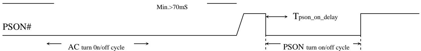
Figure 2 : Turn On/Off Timing
